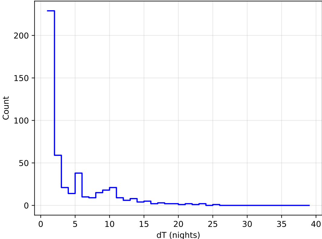
too_elab_heavy_r64_d3_gz_v3.4_10yrs all bands: DD: COSMOS Delta Nights Histogram
