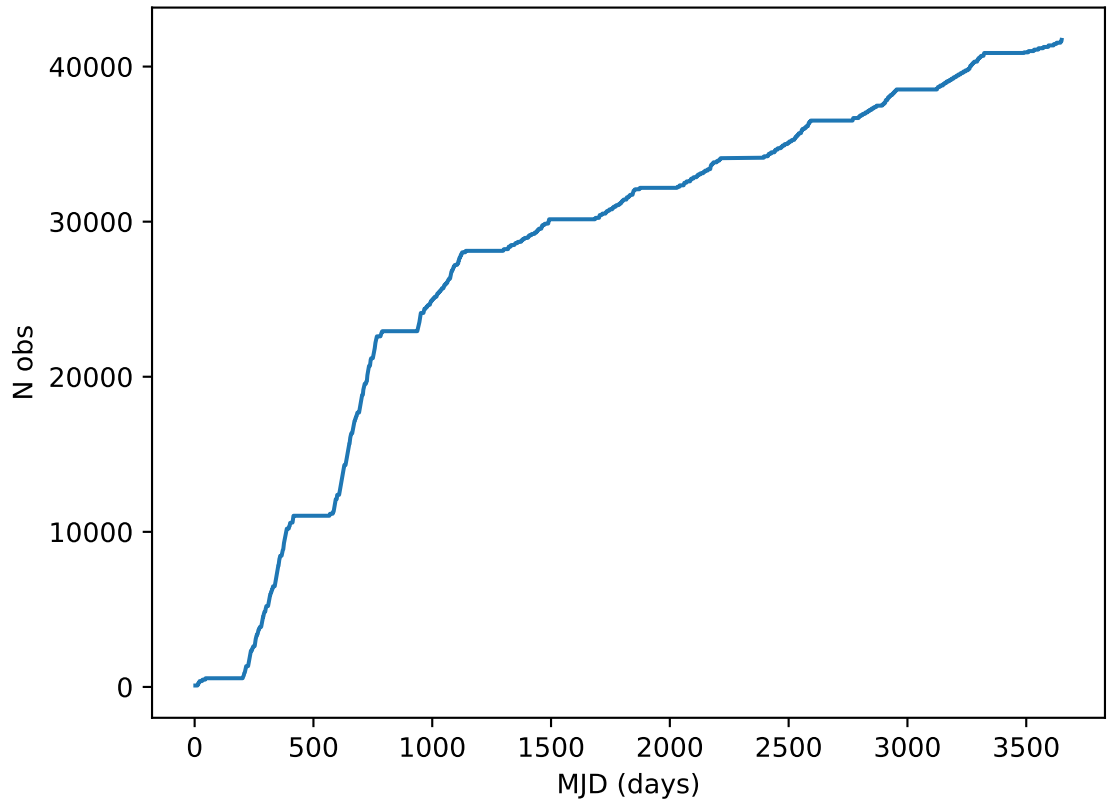
too_elab_heavy_r64_d3_gz_v3.4_10yrs all bands: DD:COSMOS Cumulative NVisits
