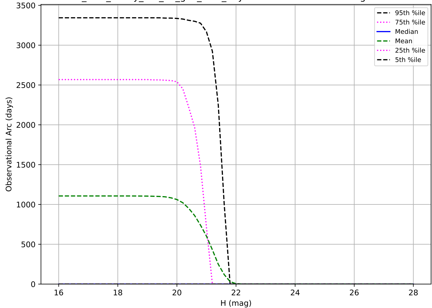
too_elab_heavy_r64_d3_griz_v3.4_10yrs: Observational Arc Length Vatra
