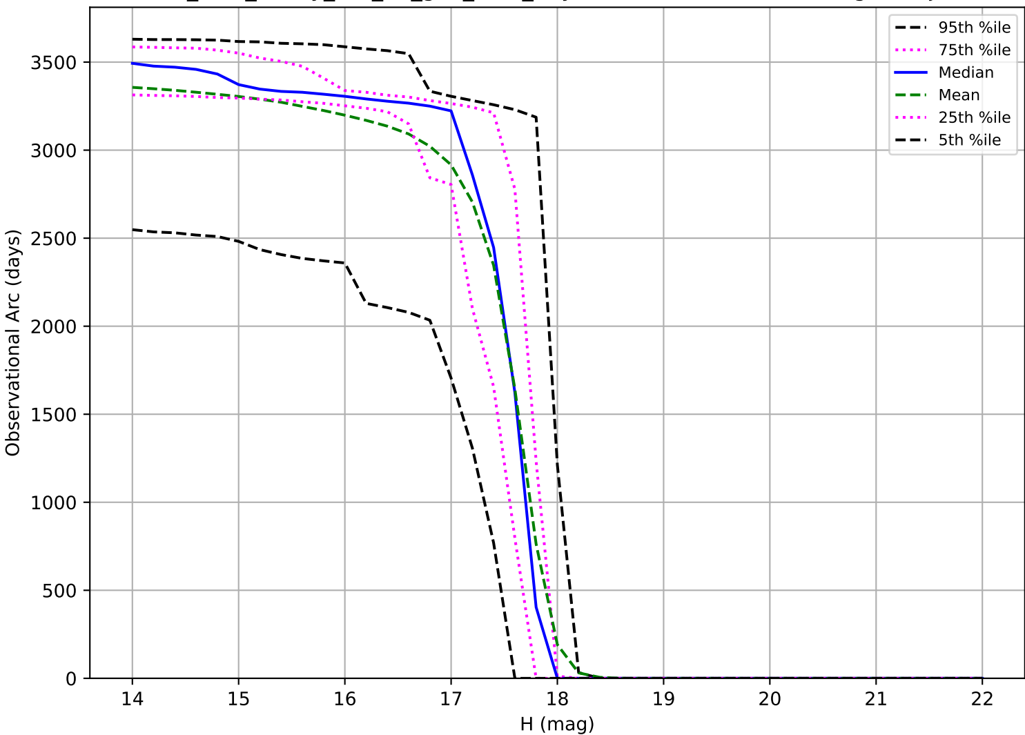
too_elab_heavy_r64_d3_griz_v3.4_10yrs: Observational Arc Length Trojan
