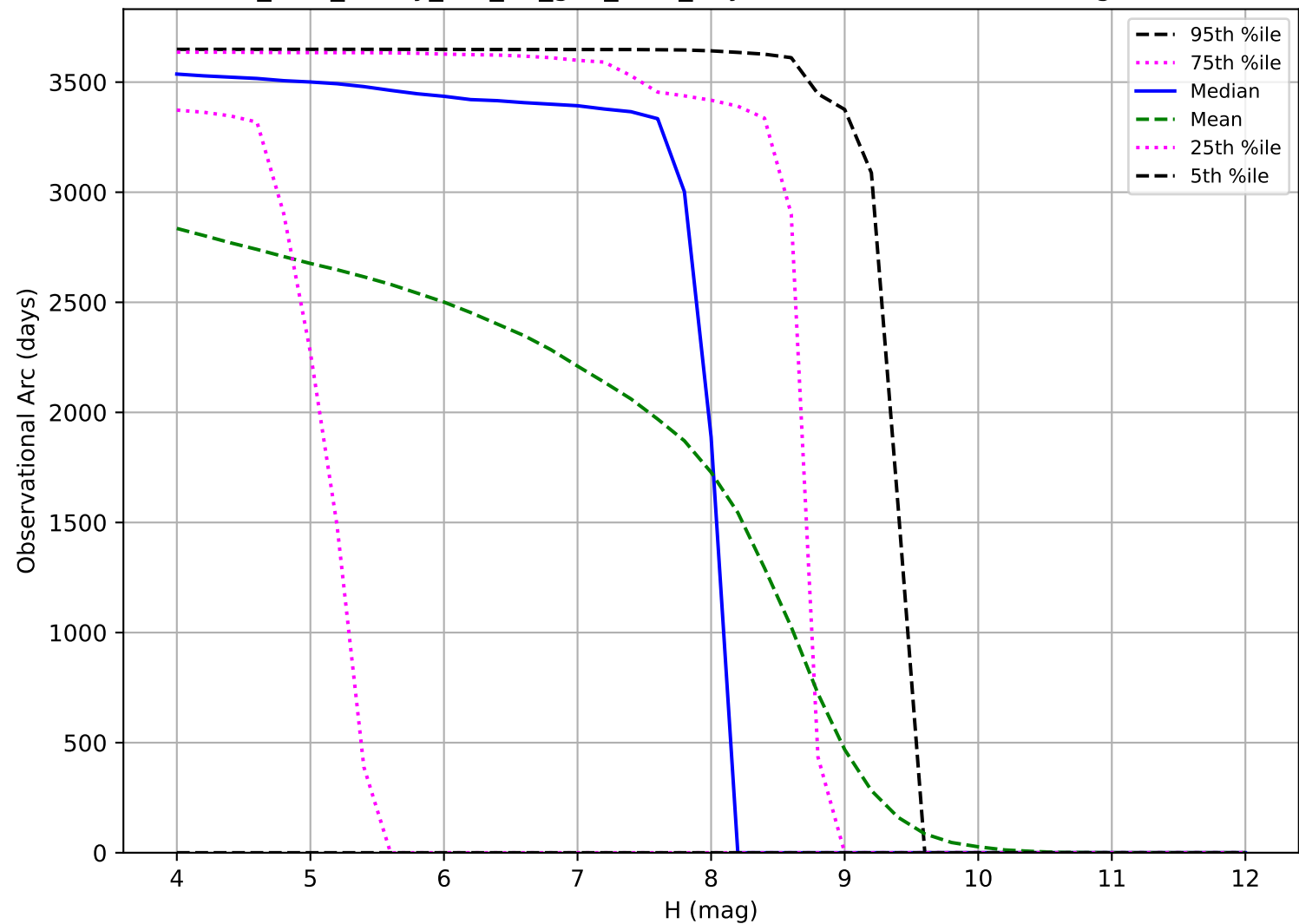
too_elab_heavy_r64_d3_griz_v3.4_10yrs: Observational Arc Length TNO
