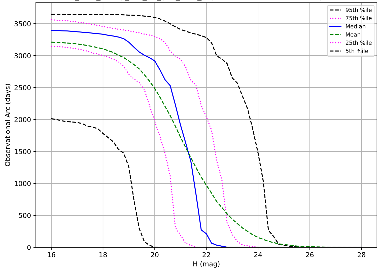
too_elab_heavy_r64_d3_griz_v3.4_10yrs: Observational Arc Length PHA
