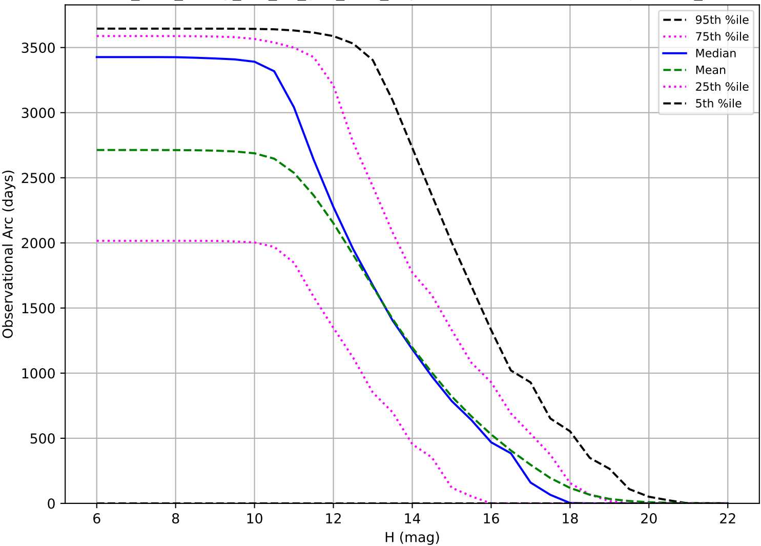
too_elab_heavy_r64_d3_griz_v3.4_10yrs: Observational Arc Length OCC_r5
