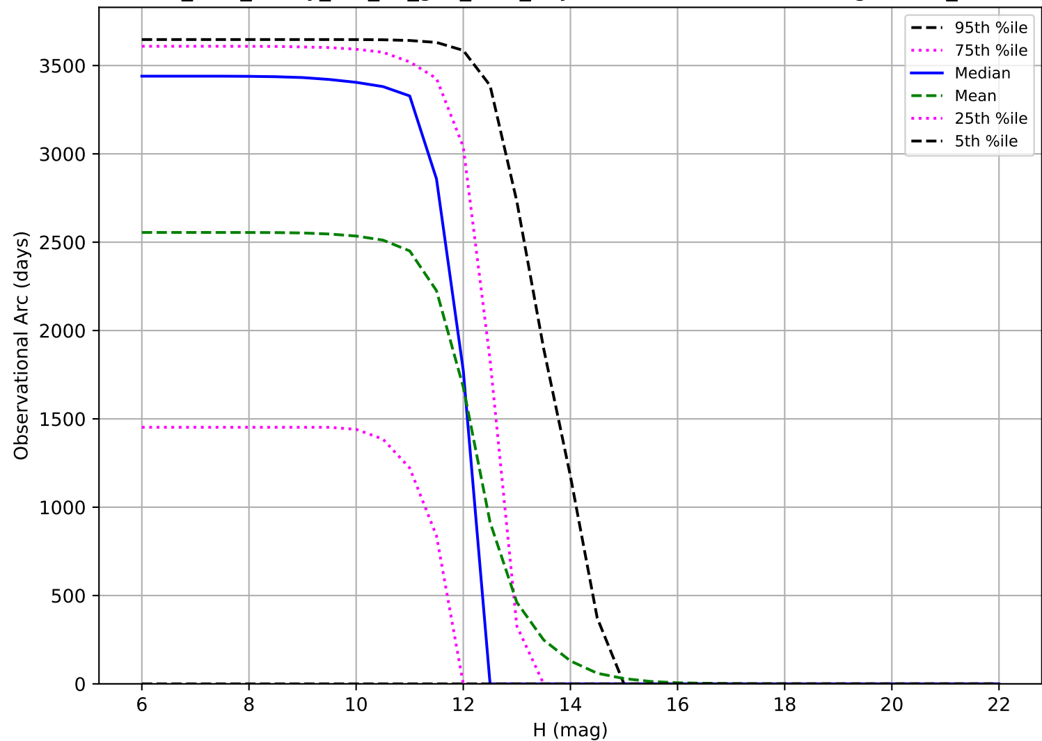
too_elab_heavy_r64_d3_griz_v3.4_10yrs: Observational Arc Length OCC_r20
