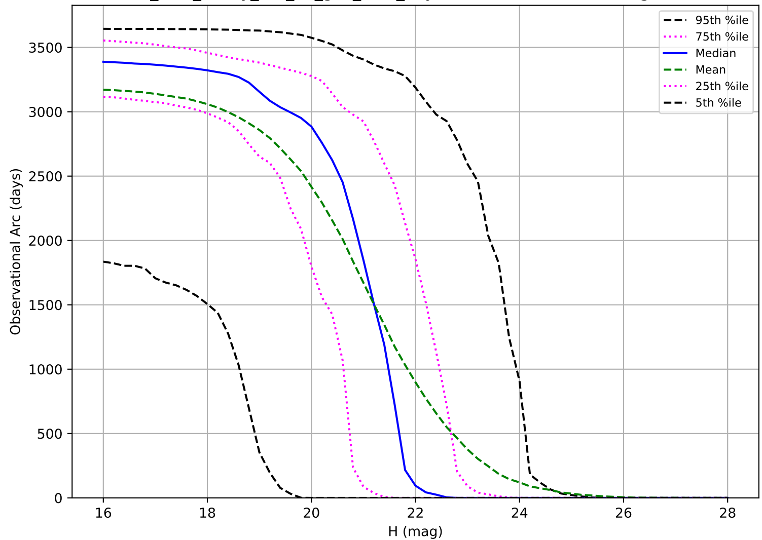
too_elab_heavy_r64_d3_griz_v3.4_10yrs: Observational Arc Length NEO
