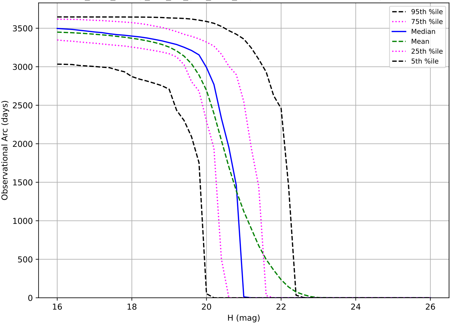
too_elab_heavy_r64_d3_griz_v3.4_10yrs: Observational Arc Length MBA
