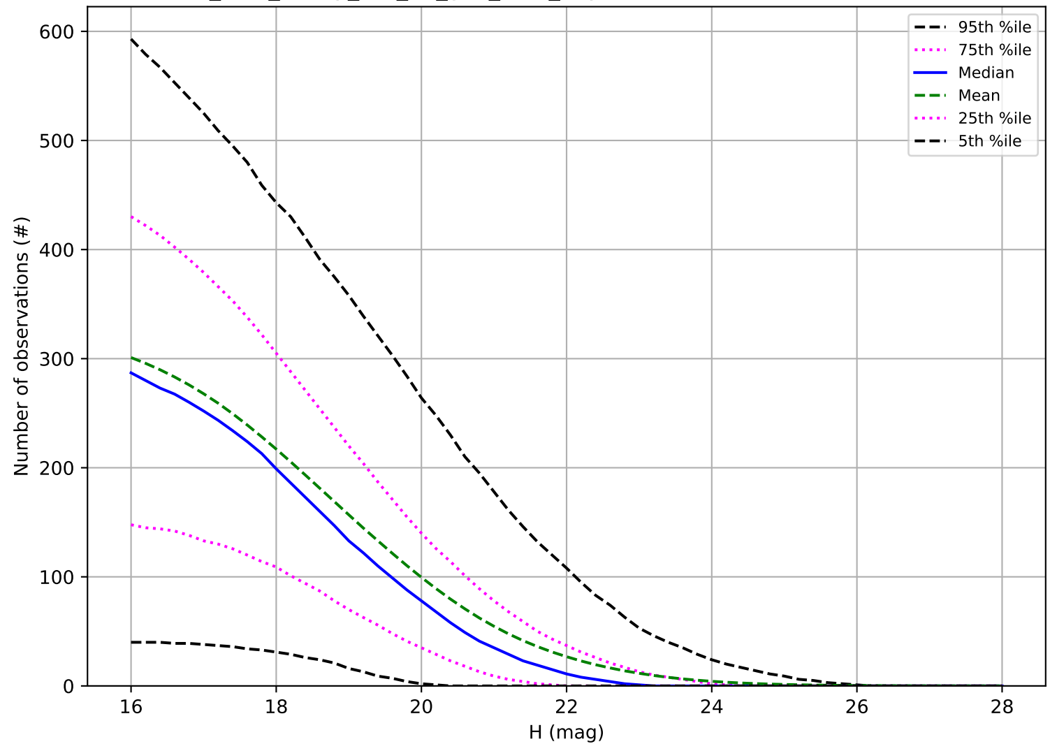
too_elab_heavy_r64_d3_griz_v3.4_10yrs: Number of observations PHA
