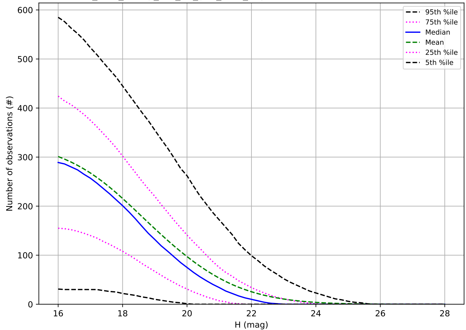
too_elab_heavy_r64_d3_griz_v3.4_10yrs: Number of observations NEO
