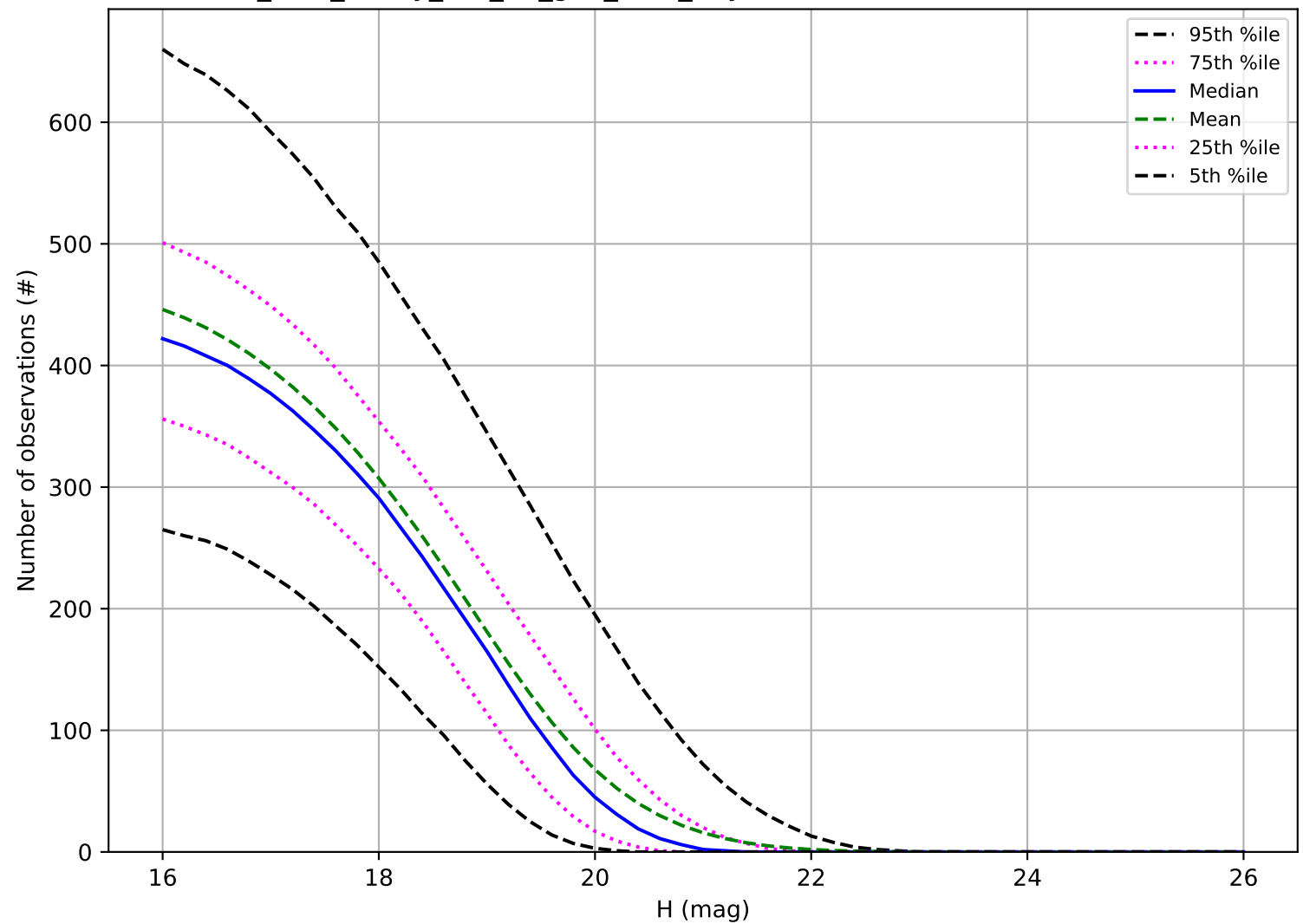
too_elab_heavy_r64_d3_griz_v3.4_10yrs: Number of observations MBA
