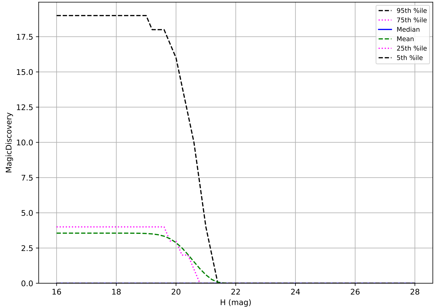
too_elab_heavy_r64_d3_griz_v3.4_10yrs: Vatira 6 detections in 60 nights detection loss
