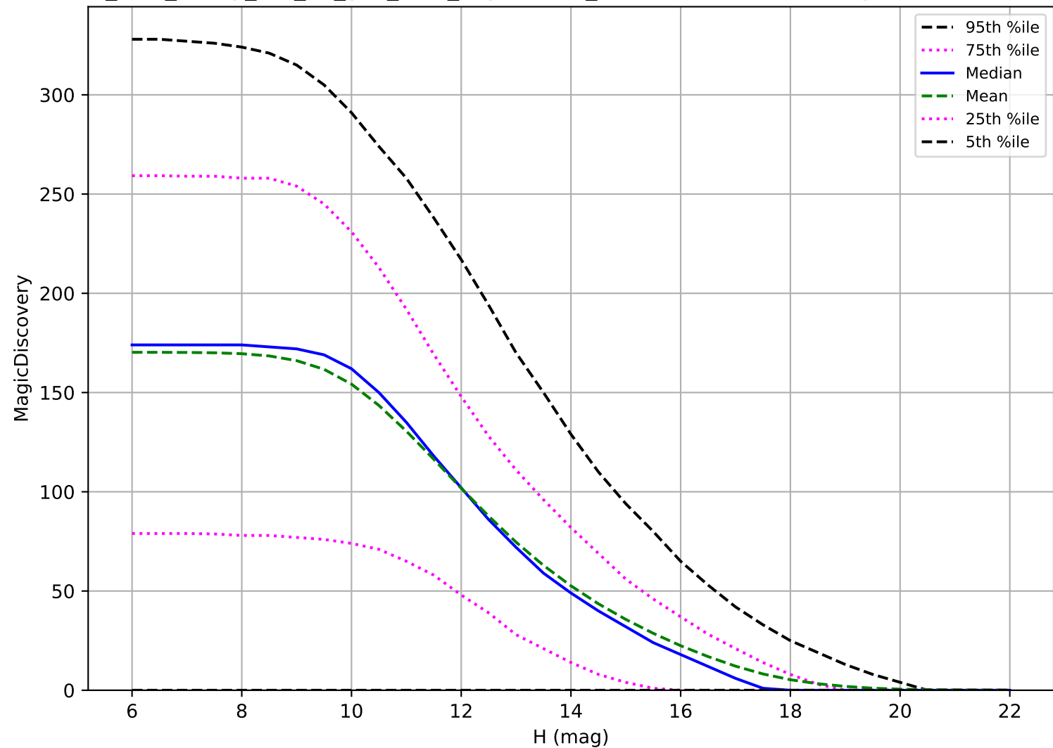
too_elab_heavy_r64_d3_griz_v3.4_10yrs: OCC_r5 6 detections in 60 nights detection loss
