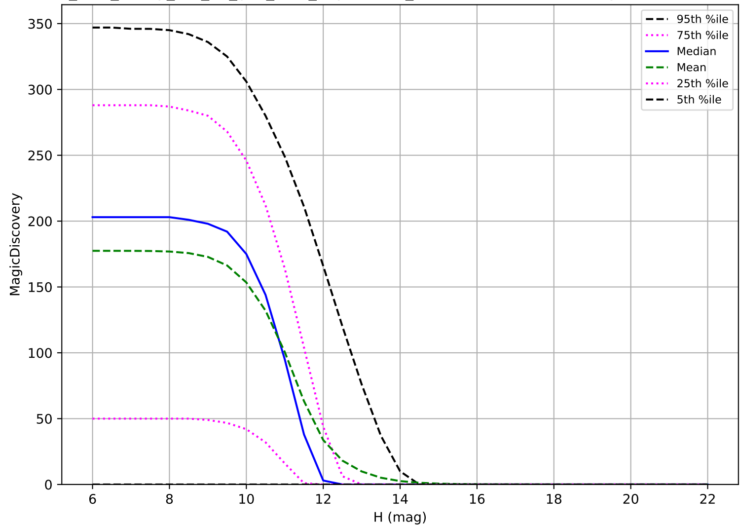
too_elab_heavy_r64_d3_griz_v3.4_10yrs: OCC_r20 6 detections in 60 nights detection loss
