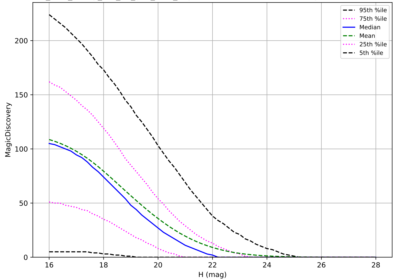
too_elab_heavy_r64_d3_griz_v3.4_10yrs: NEO 6 detections in 60 nights detection loss
