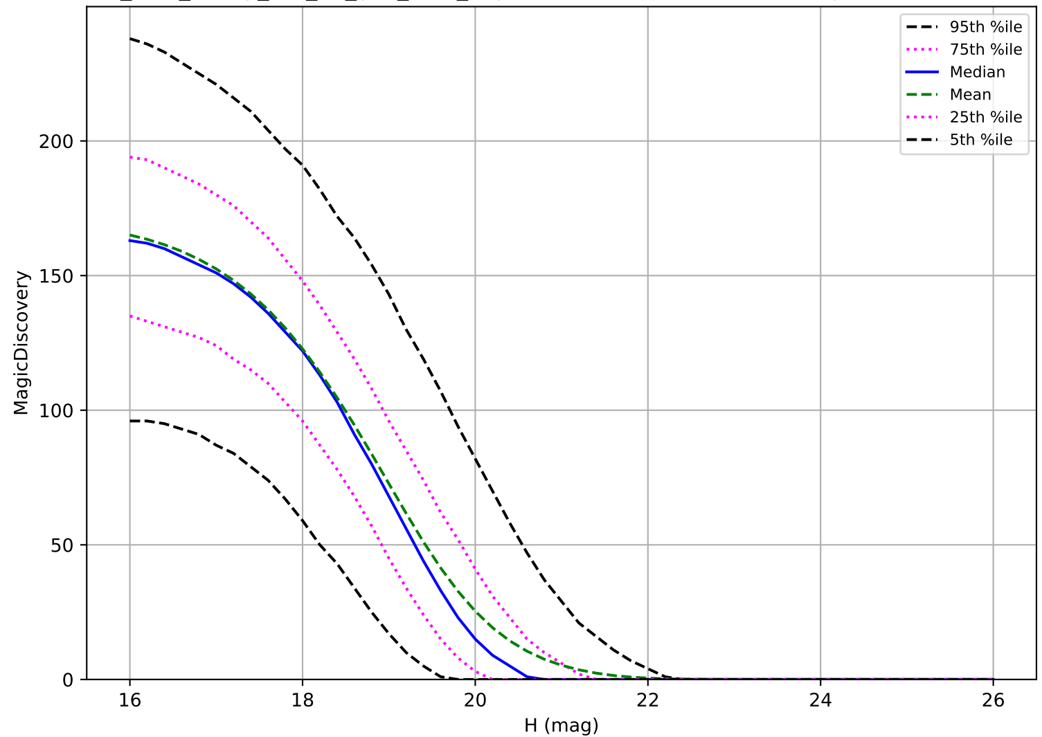
too_elab_heavy_r64_d3_griz_v3.4_10yrs: MBA 6 detections in 60 nights detection loss
