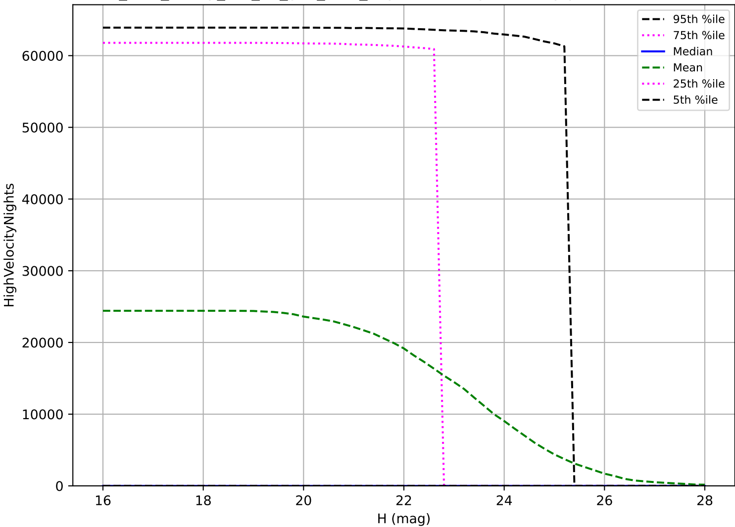
too_elab_heavy_r64_d3_griz_v3.4_10yrs: PHA High velocity pair detection loss
