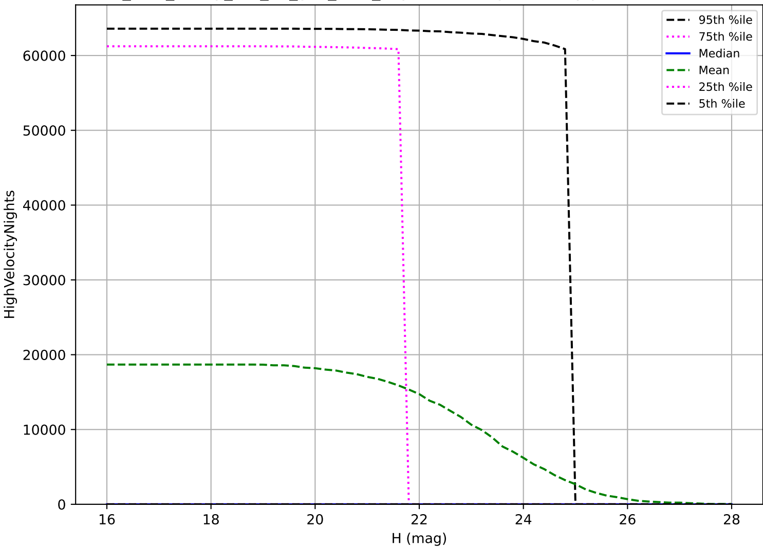
too_elab_heavy_r64_d3_griz_v3.4_10yrs: NEO High velocity pair detection loss
