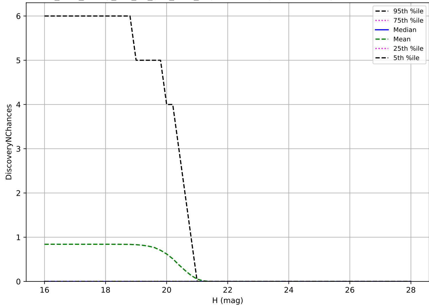
too_elab_heavy_r64_d3_griz_v3.4_10yrs: Vatira 3 pairs in 15 nights detection loss
