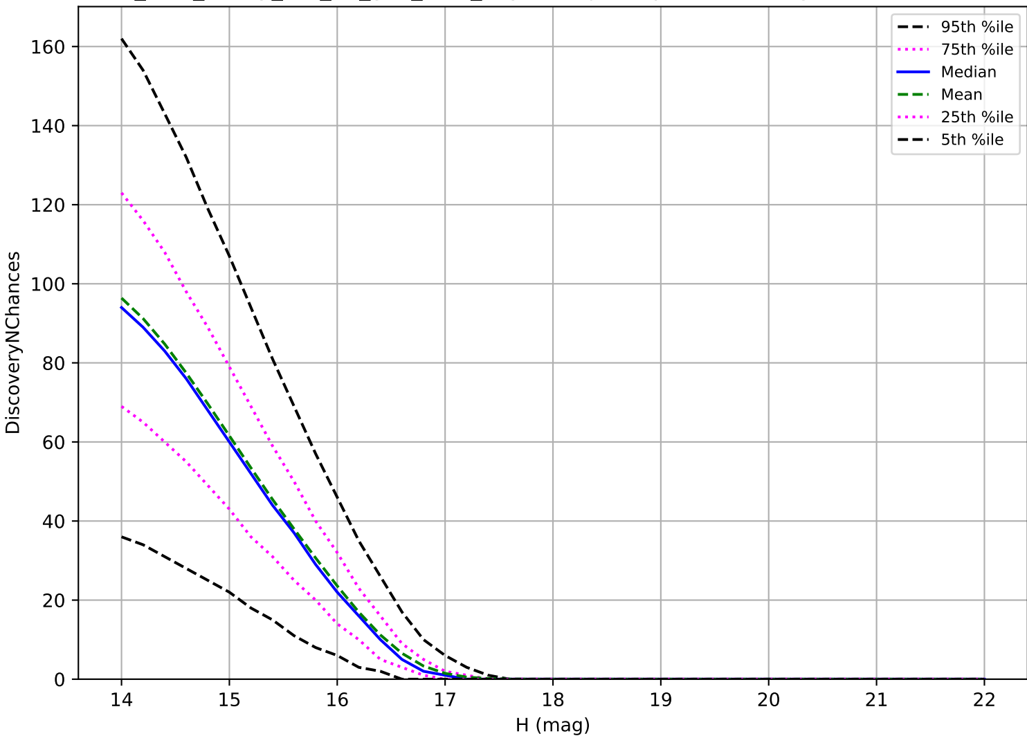
too_elab_heavy_r64_d3_griz_v3.4_10yrs: Trojan 3 pairs in 15 nights detection loss
