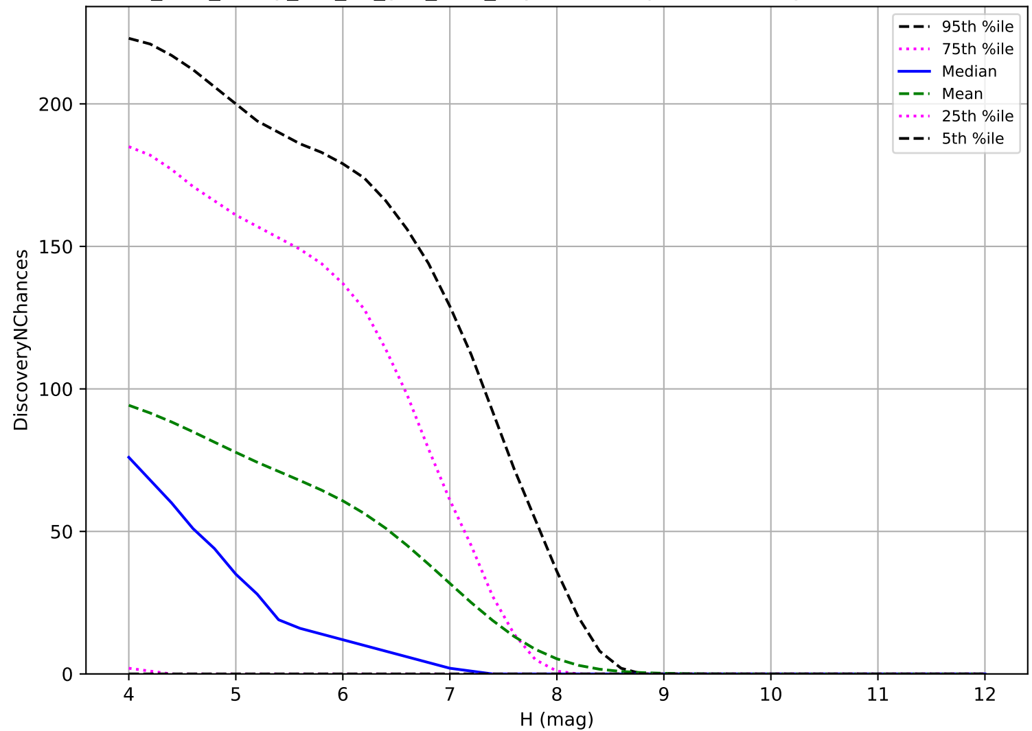
too_elab_heavy_r64_d3_griz_v3.4_10yrs: TNO 3 pairs in 15 nights detection loss
