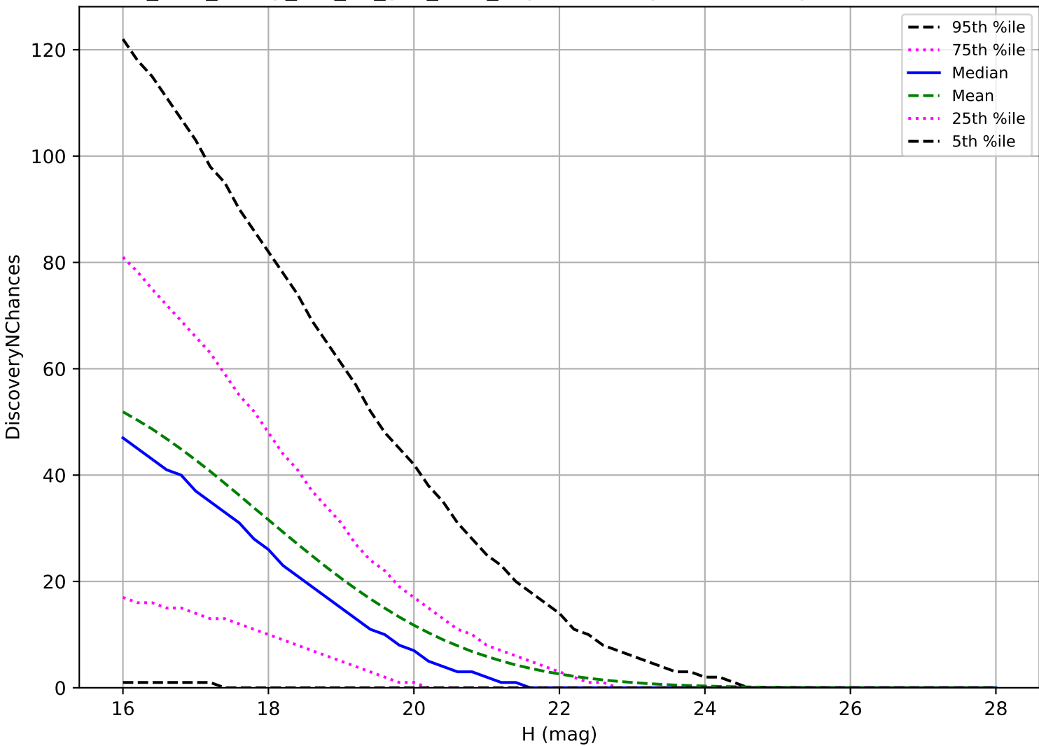
too_elab_heavy_r64_d3_griz_v3.4_10yrs: PHA 3 pairs in 15 nights detection loss
