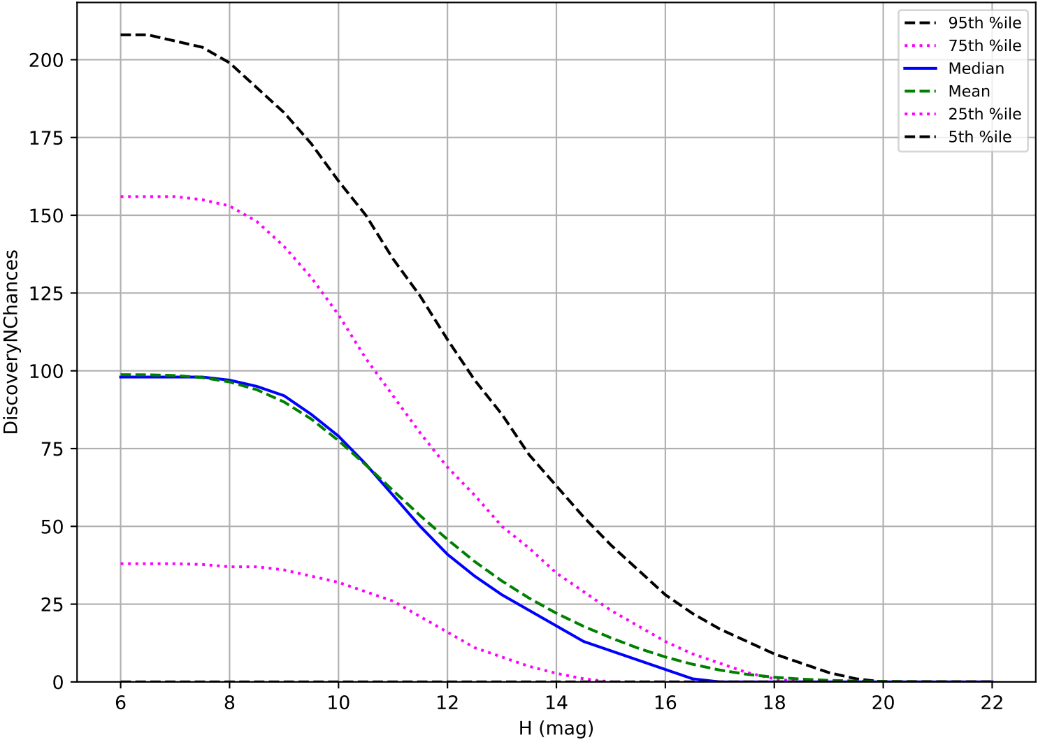
too_elab_heavy_r64_d3_griz_v3.4_10yrs: OCC_r5 3 pairs in 15 nights detection loss
