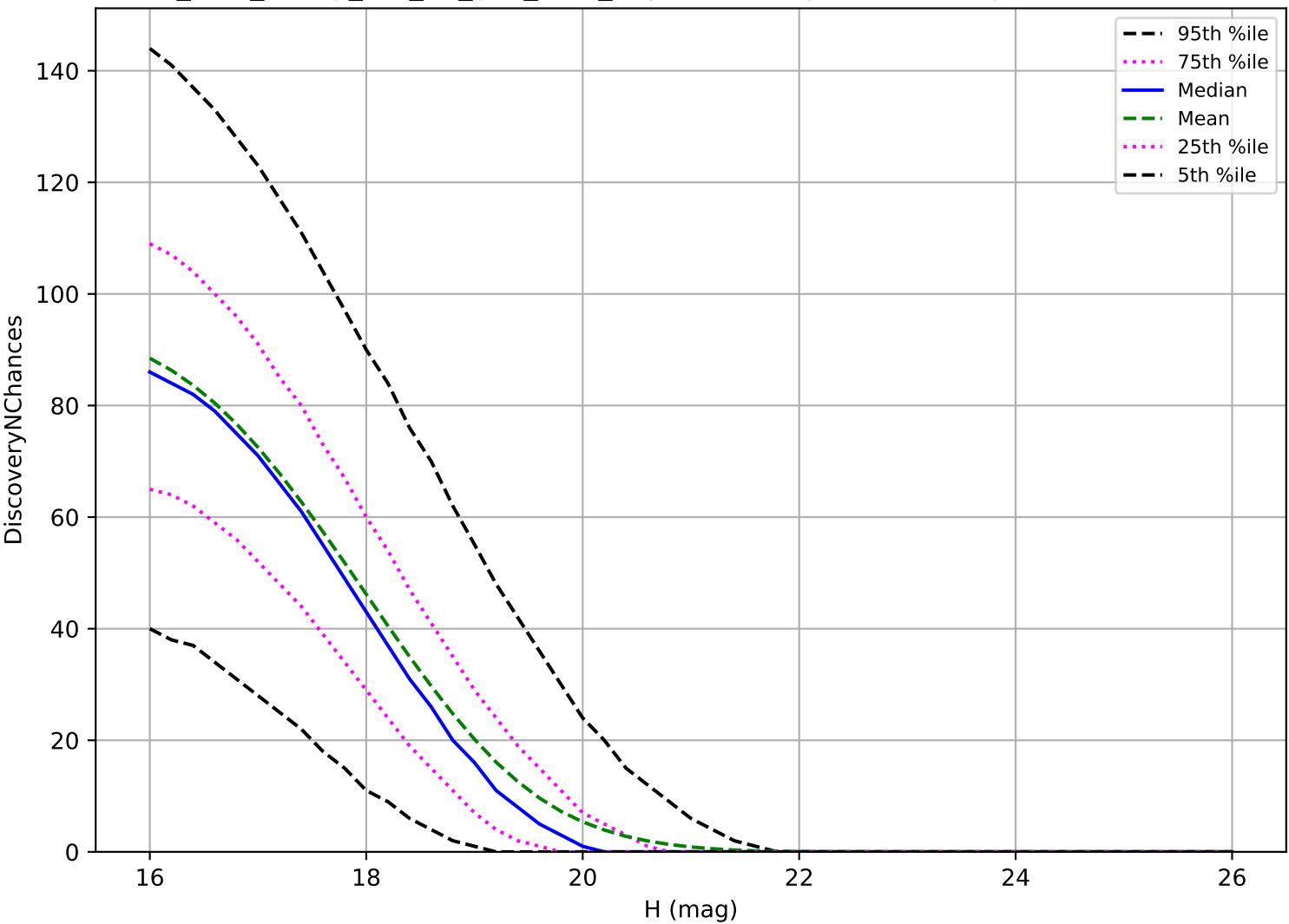
too_elab_heavy_r64_d3_griz_v3.4_10yrs: MBA 3 pairs in 15 nights detection loss
