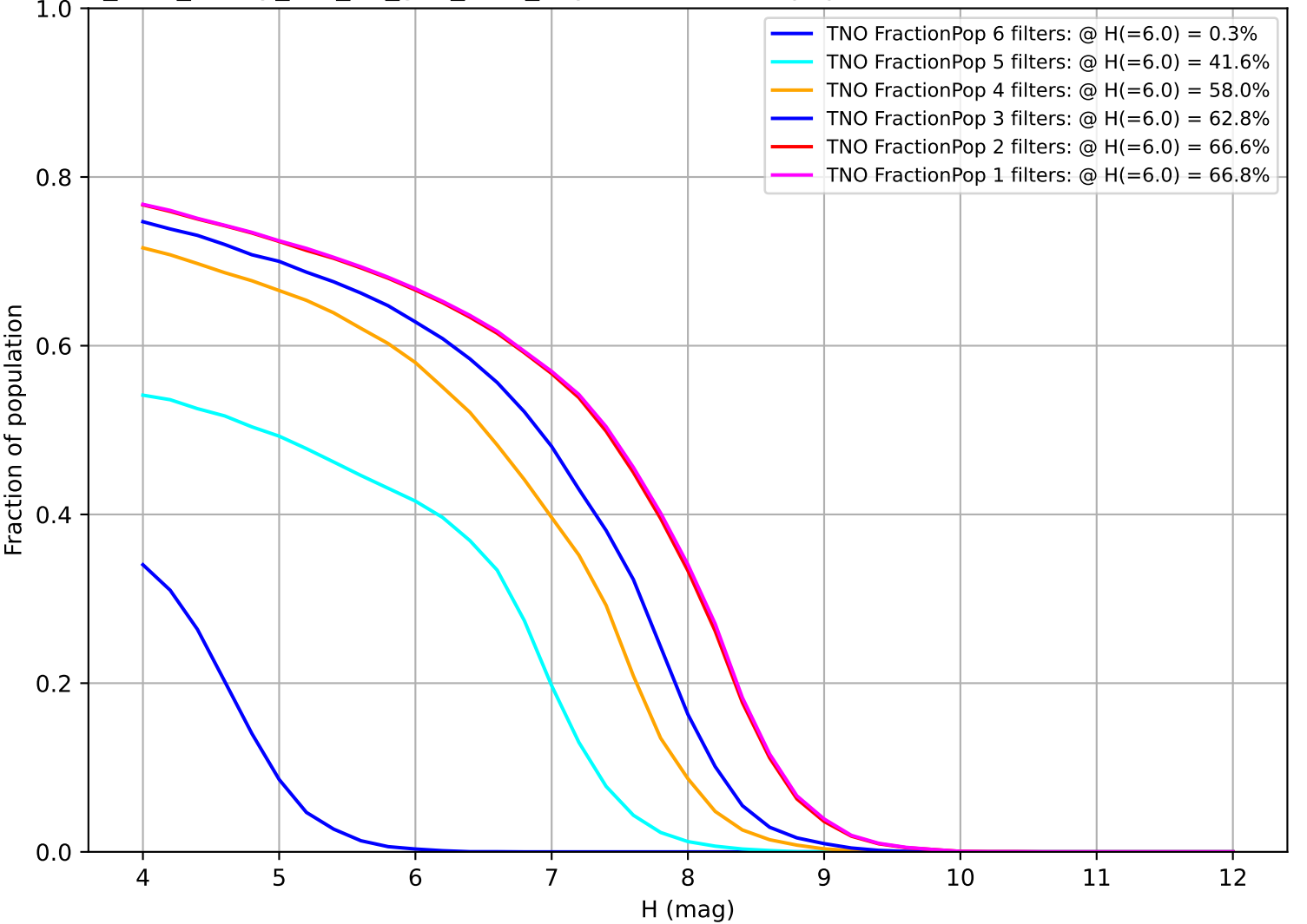
too_elab_heavy_r64_d3_griz_v3.4_10yrs: Fraction of population with colors in X filters TNO
