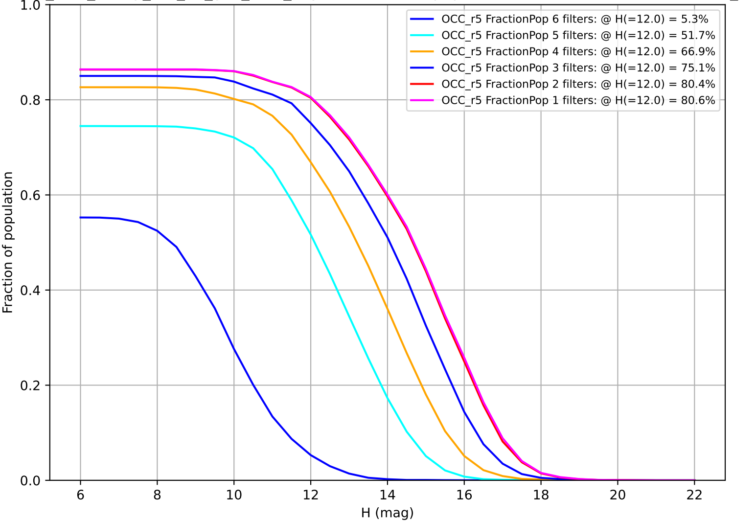
too_elab_heavy_r64_d3_griz_v3.4_10yrs: Fraction of population with colors in X filters OCC_r5
