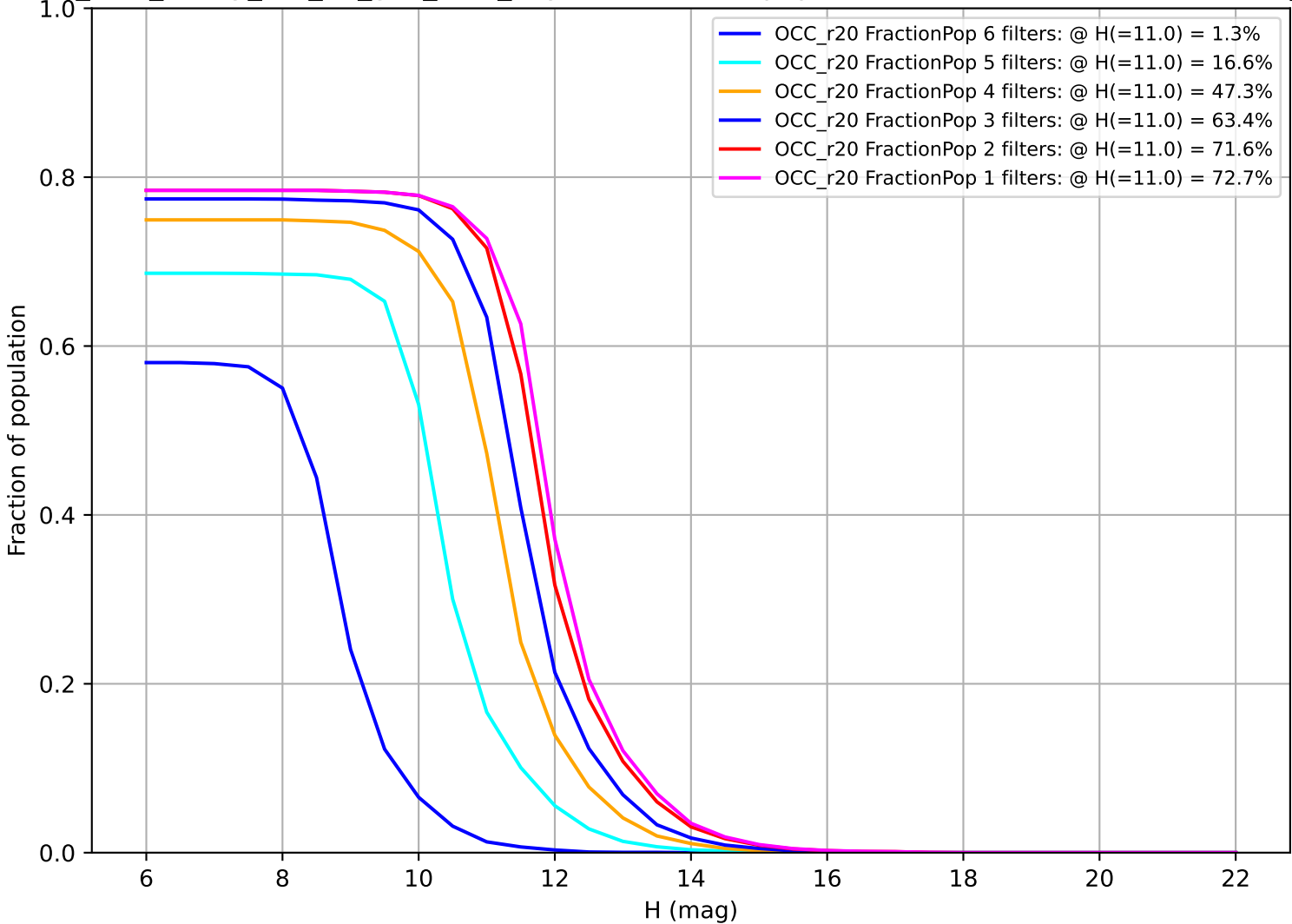
too_elab_heavy_r64_d3_griz_v3.4_10yrs: Fraction of population with colors in X filters OCC_r20
