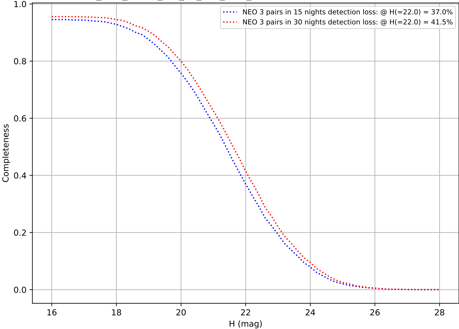
too_elab_heavy_r64_d3_griz_v3.4_10yrs: DifferentialCompleteness
