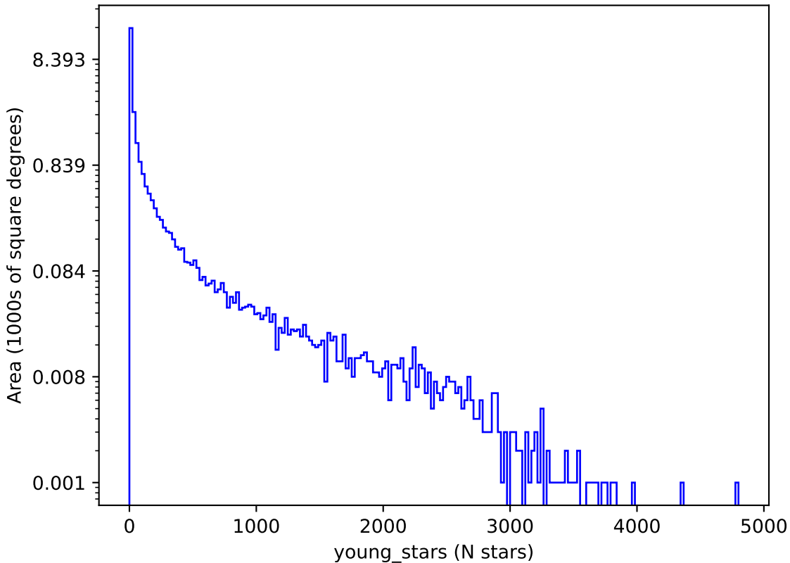
too_elab_heavy_r64_d3_griz_v3.4_10yrs : young_stars
