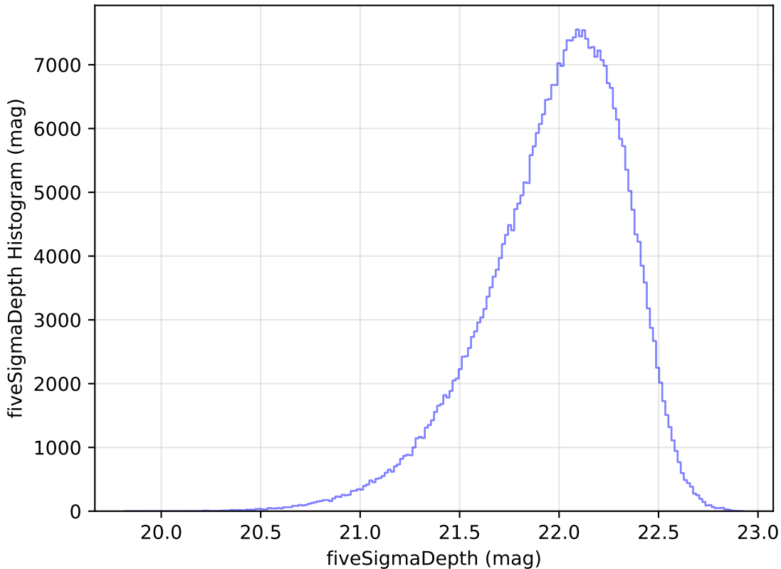
too_elab_heavy_r64_d3_griz_v3.4_10yrs y: fiveSigmaDepth Histogram
