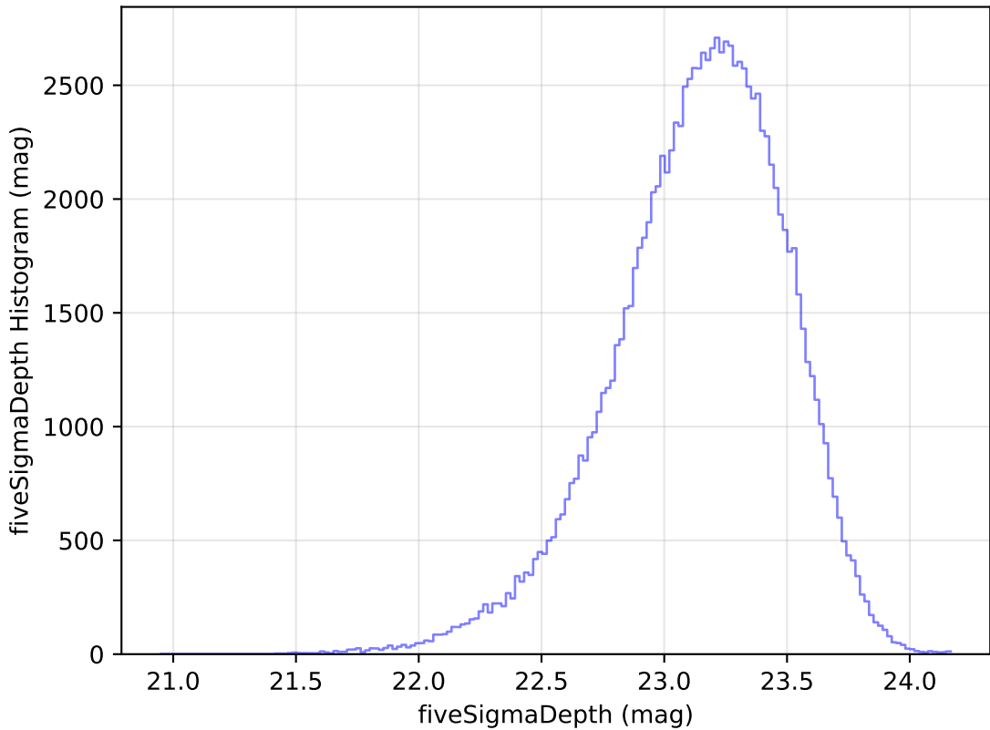
too_elab_heavy_r64_d3_griz_v3.4_10yrs u: fiveSigmaDepth Histogram
