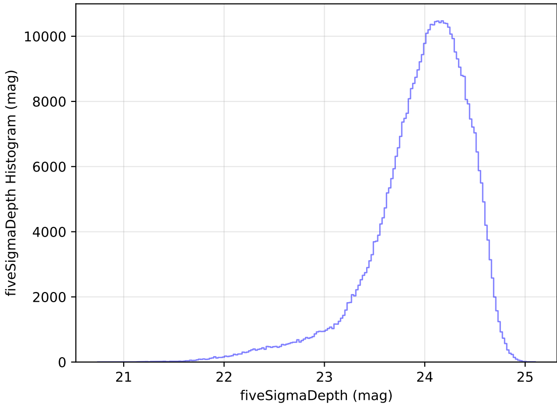
too_elab_heavy_r64_d3_griz_v3.4_10yrs r: fiveSigmaDepth Histogram
