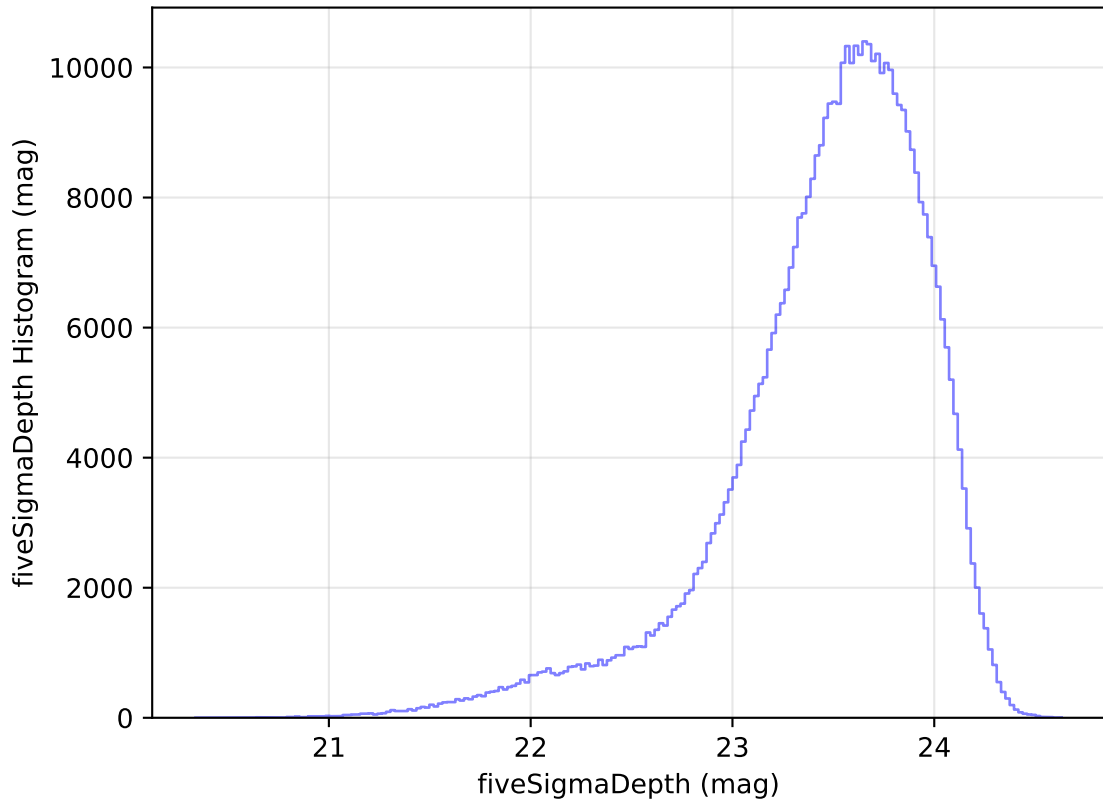
too_elab_heavy_r64_d3_griz_v3.4_10yrs i: fiveSigmaDepth Histogram
