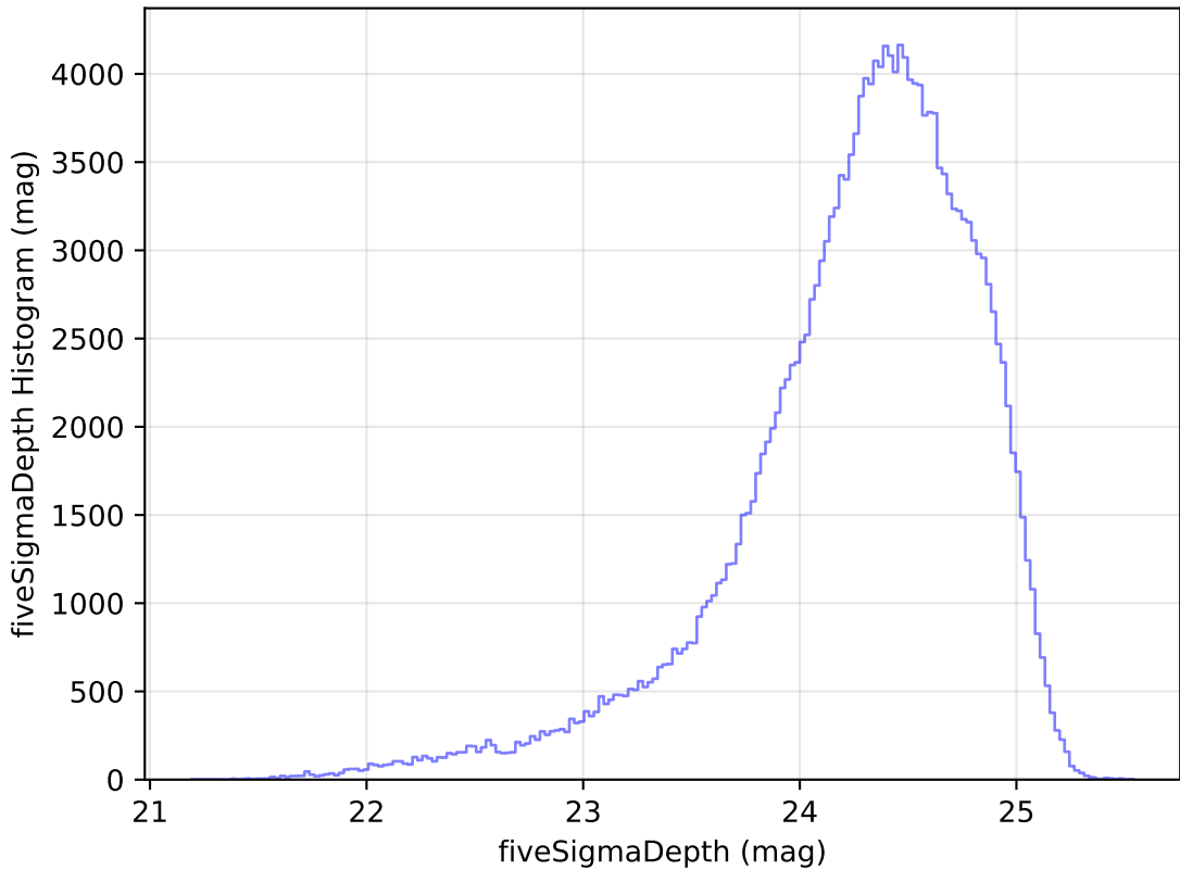
too_elab_heavy_r64_d3_griz_v3.4_10yrs g: fiveSigmaDepth Histogram
