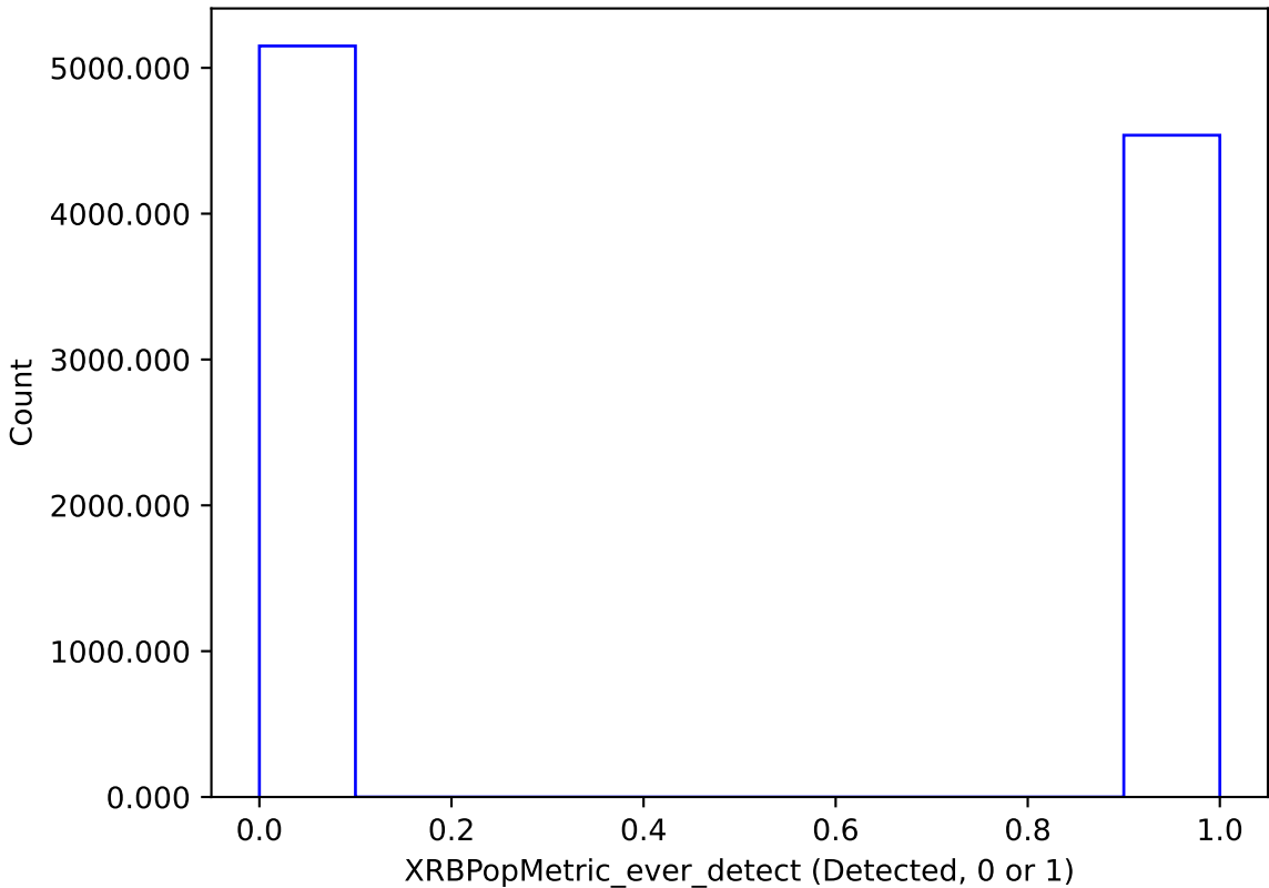
too_elab_heavy_r64_d3_griz_v3.4_10yrs : XRBPopMetric_ever_detect
