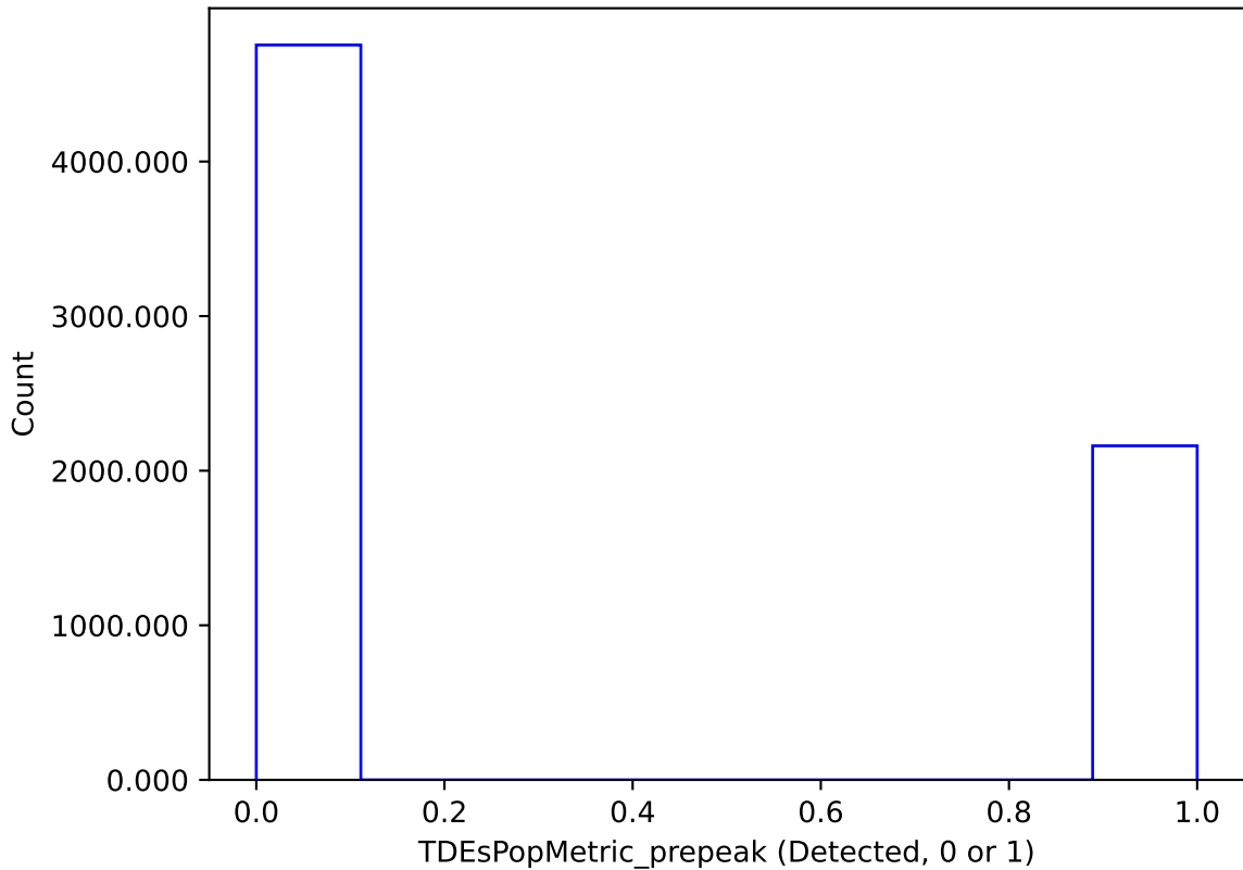
too_elab_heavy_r64_d3_griz_v3.4_10yrs : TDEsPopMetric_prepeak
