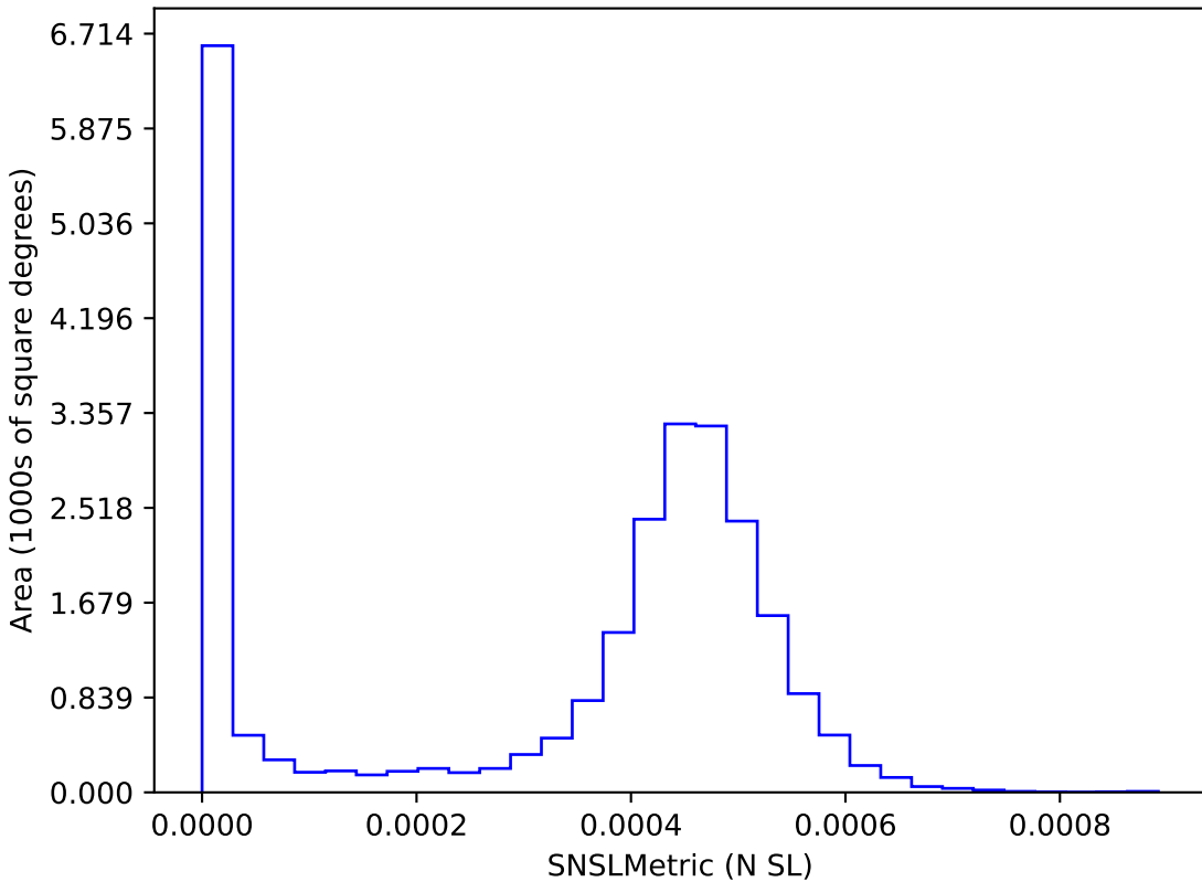
too_elab_heavy_r64_d3_griz_v3.4_10yrs : SNSLMetric
