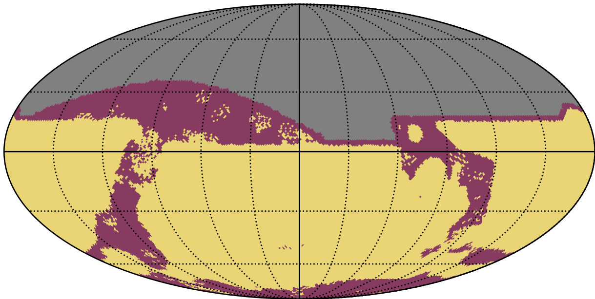
too_elab_heavy_r64_d3_griz_v3.4_10yrs : RapidRevisits
