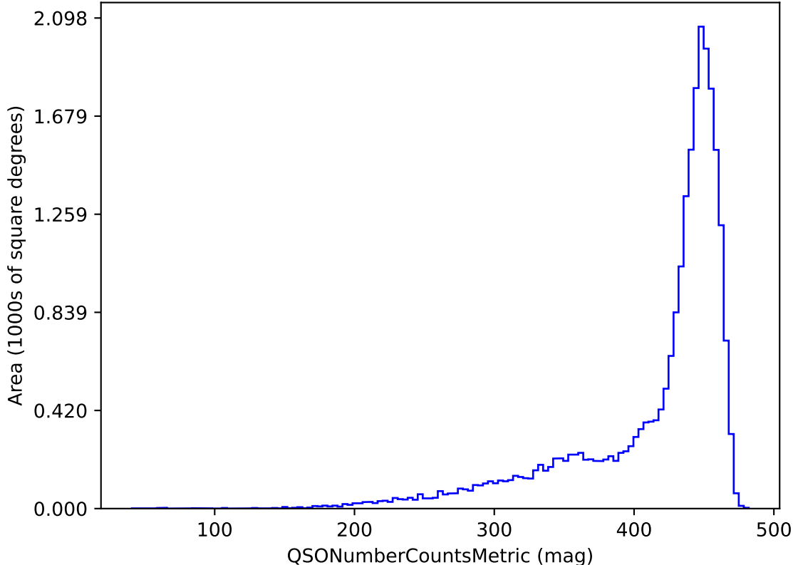
too_elab_heavy_r64_d3_griz_v3.4_10yrs g band and non-DD: QSONumberCountsMetric
