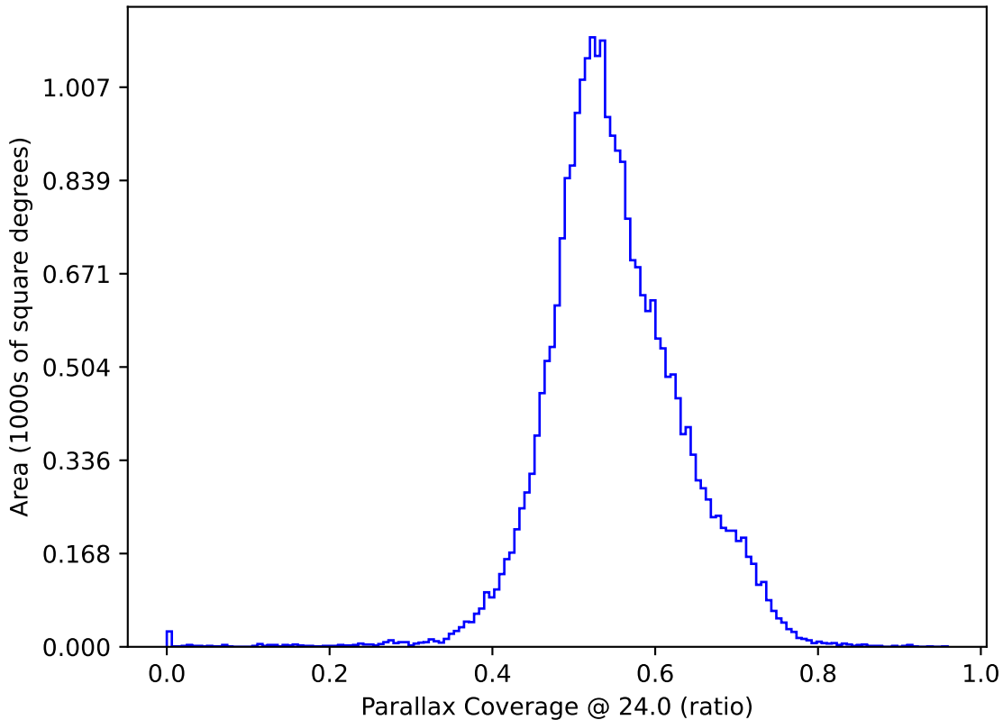
too_elab_heavy_r64_d3_griz_v3.4_10yrs : Parallax Coverage @ 24.0
