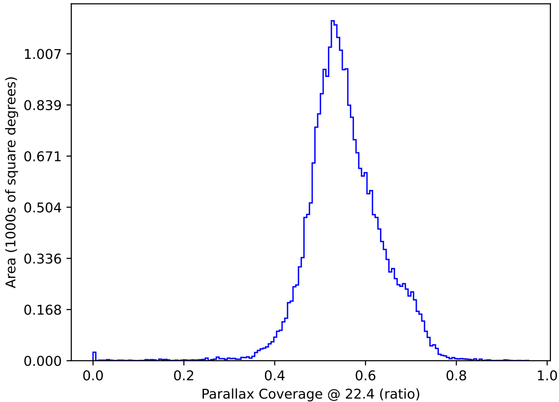
too_elab_heavy_r64_d3_griz_v3.4_10yrs : Parallax Coverage @ 22.4
