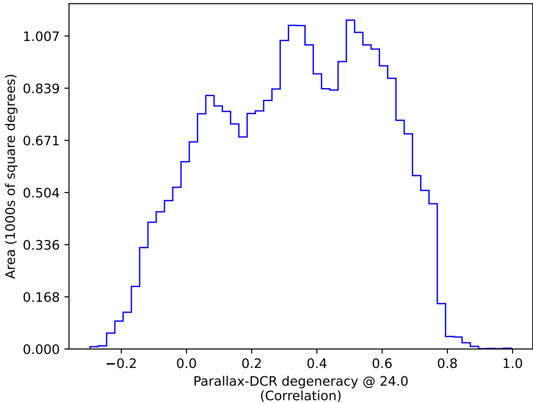
too_elab_heavy_r64_d3_griz_v3.4_10yrs : Parallax-DCR degeneracy @ 24.0
