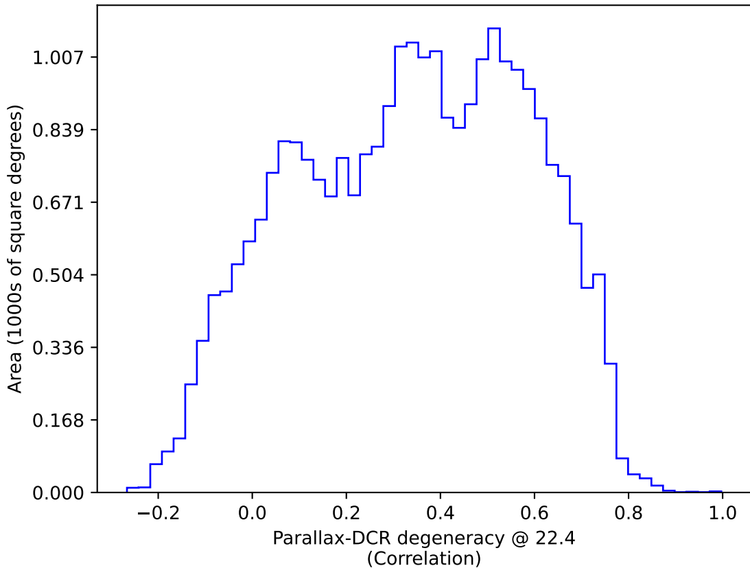
too_elab_heavy_r64_d3_griz_v3.4_10yrs : Parallax-DCR degeneracy @ 22.4
