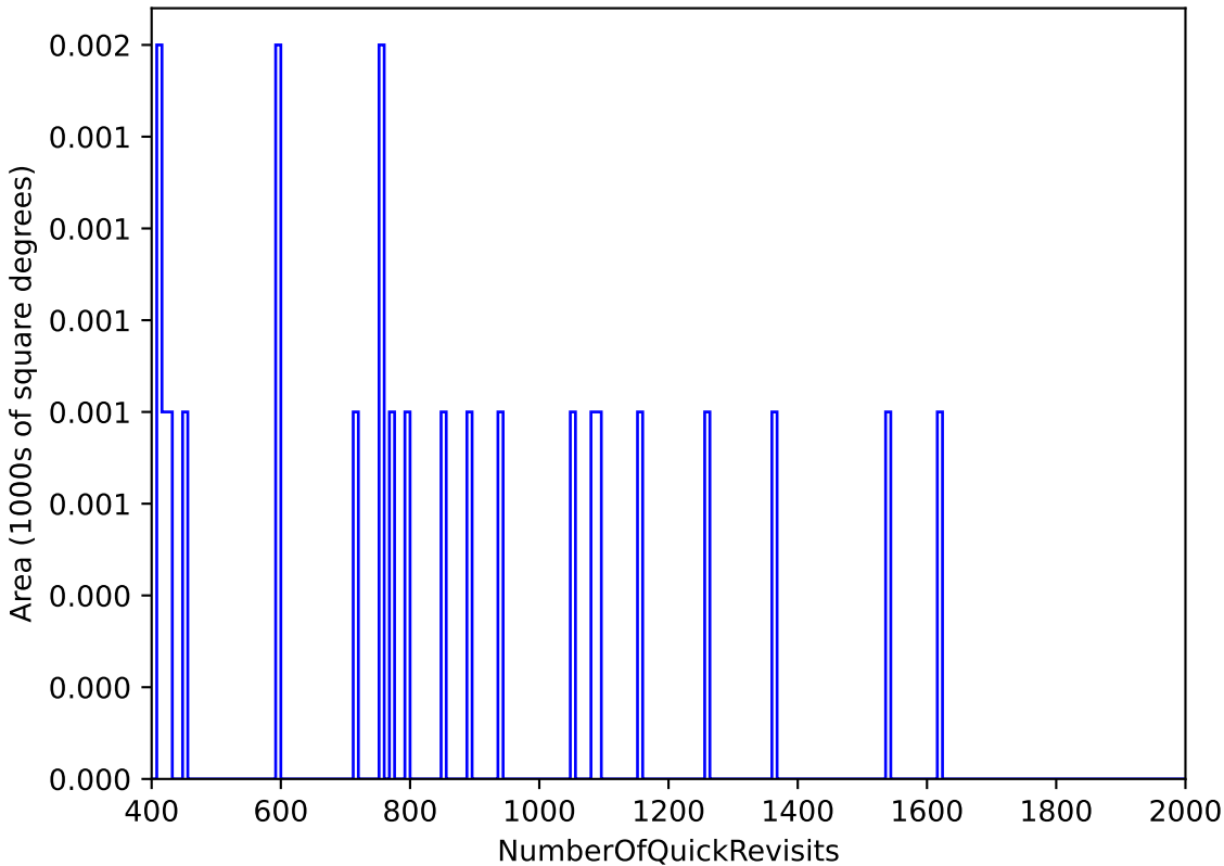
too_elab_heavy_r64_d3_griz_v3.4_10yrs : NumberOfQuickRevisits
