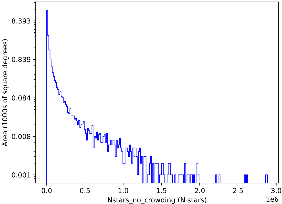
too_elab_heavy_r64_d3_griz_v3.4_10yrs u: Nstars_no_crowding
