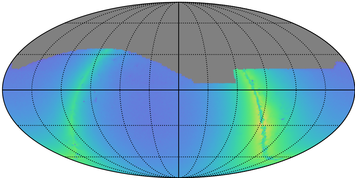
too_elab_heavy_r64_d3_griz_v3.4_10yrs i: Nstars_no_crowding
