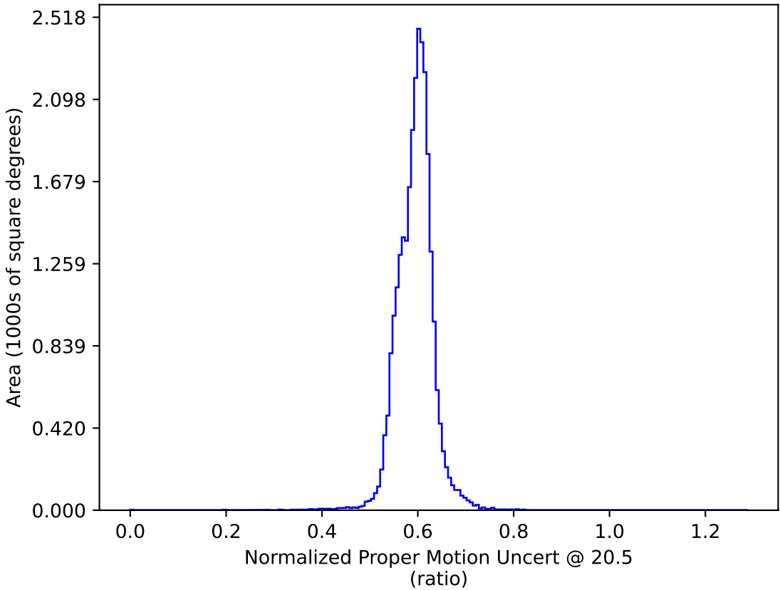
too_elab_heavy_r64_d3_griz_v3.4_10yrs : Normalized Proper Motion Uncert @ 20.5
