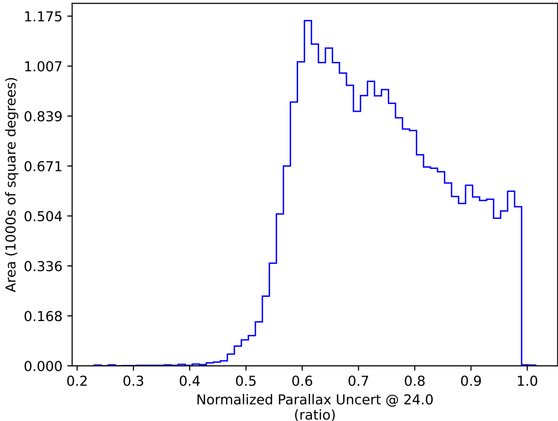
too_elab_heavy_r64_d3_griz_v3.4_10yrs : Normalized Parallax Uncert @ 24.0
